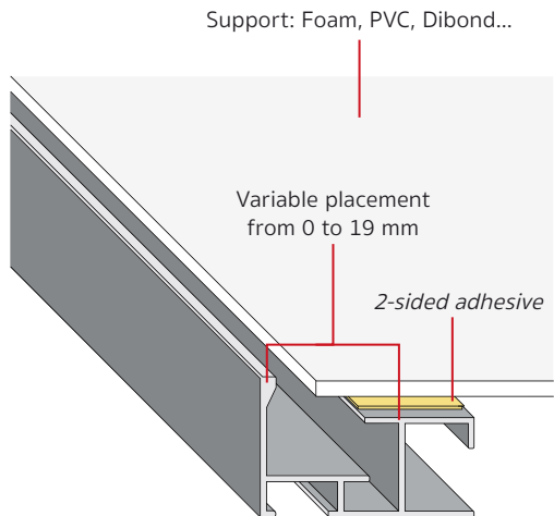
Mounting example as american box
