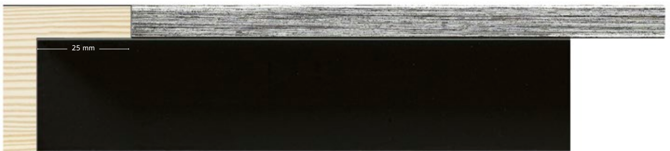
4013/33 40x35mm
