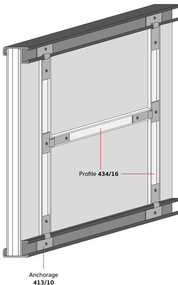
Example of mounting with profile H stabilizer
